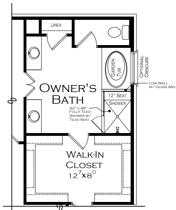
OPTIONAL OWNER'S BATH FULLY TILED SHOWER W/ 12" TILE SEAT
