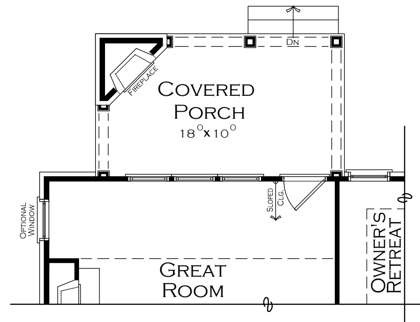
OPTIONAL COVERED PORCH WITH OPT. EXTERIOR CORNER FIREPLACE
