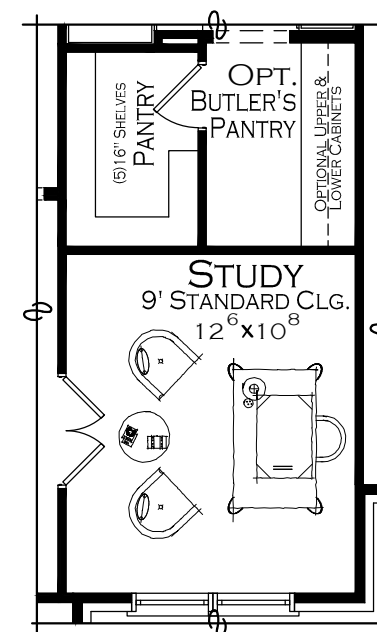
OPTIONAL STUDY IN-LIEU OF DINING ROOM WITH DOUBLE FRENCH DOORS & ENLARGED PANTRY & BUTLER'S PANTRY OPTIONAL UPPER & LOWER CABINETS IN BUTLER'S PANTRY
