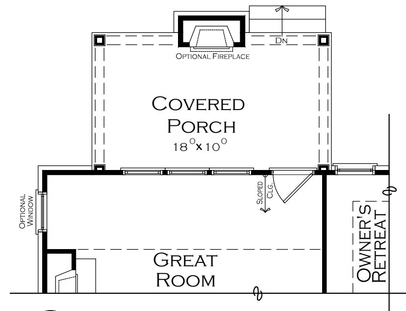
OPTIONAL COVERED PORCH WITH OPT. EXTERIOR FIREPLACE
