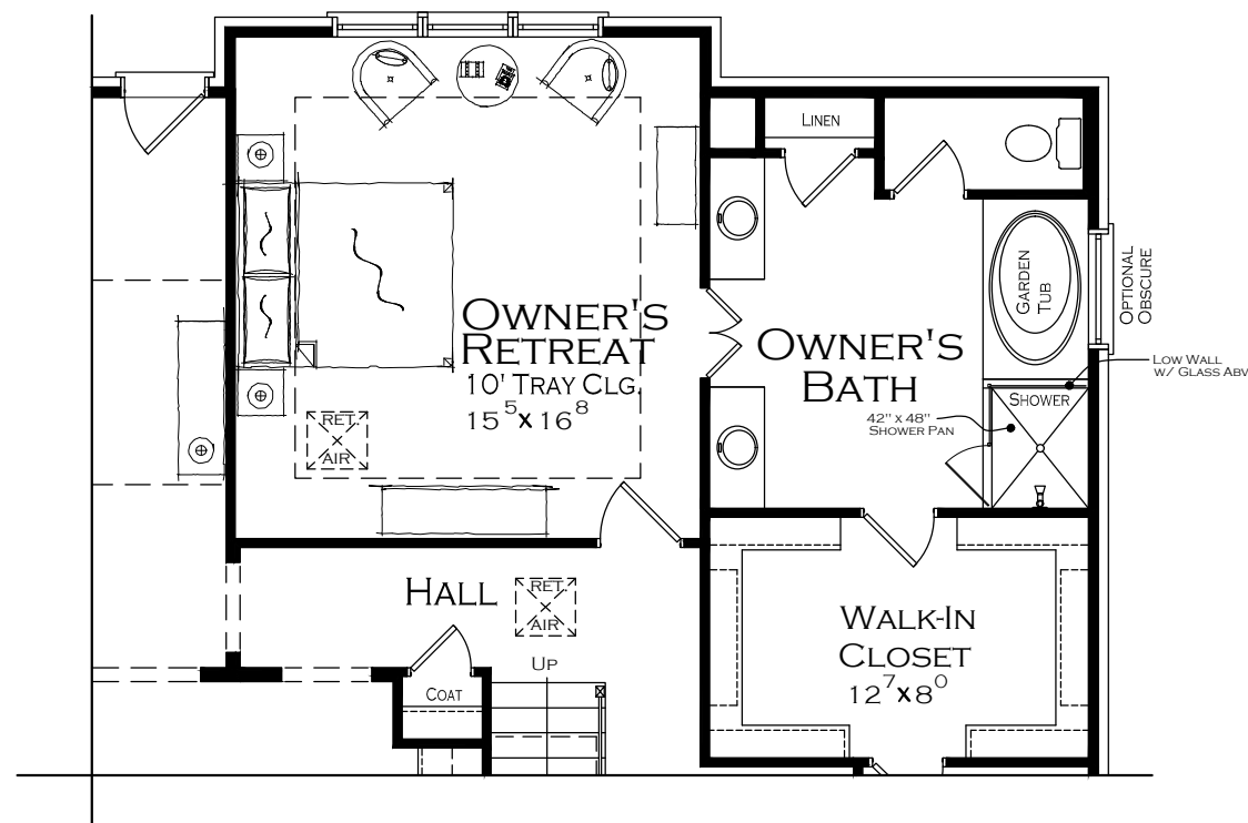
OPTIONAL ENLARGED OWNER'S RETREAT WITH 2' EXTENSION ADDITIONAL 32 SQ. FT.
