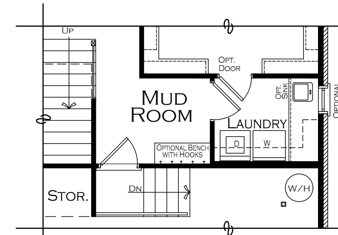
OPT. LAUNDRY OPTIONAL CABINETS & COUNTERTOP OPTIONAL SINK
