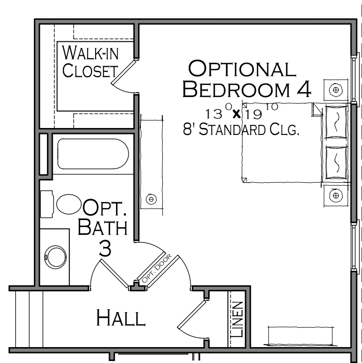
OPT. BEDROOM 4 CLOSET OPTION ADD 43 SQ FT
