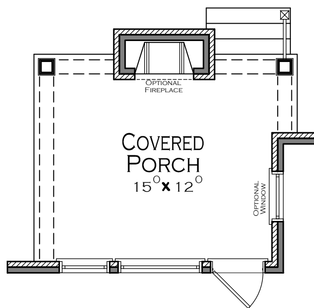
OPTIONAL REAR COVER PORCH ADD 180 SQ FT SHOWN WITH OPTIONAL FIREPLACE
