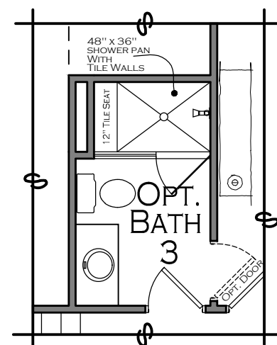
OPT. BATH 3 SHOWER OPT. #2 INCLUDES ACRYLIC PAN WITH TILE WALLS & TILE SEAT OPTIONAL TILE SHOWER FLOOR ADD 5 SQ FT
