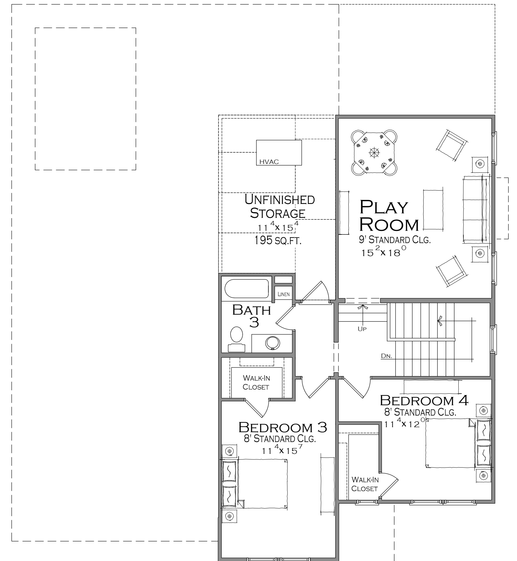
UPPER LEVEL
