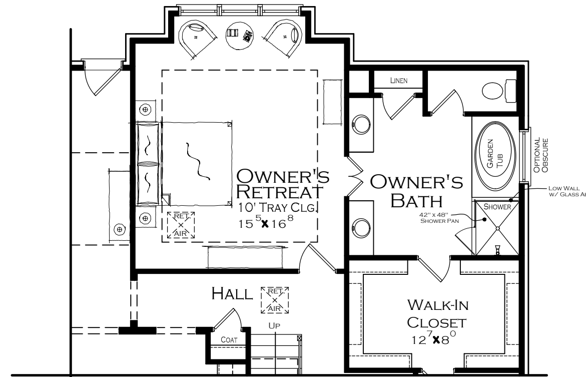
OPTIONAL ENLARGED OWNER'S RETREAT WITH SITTING AREA WITH 2' EXTENSION ADDITIONAL 53 SQ. FT.
