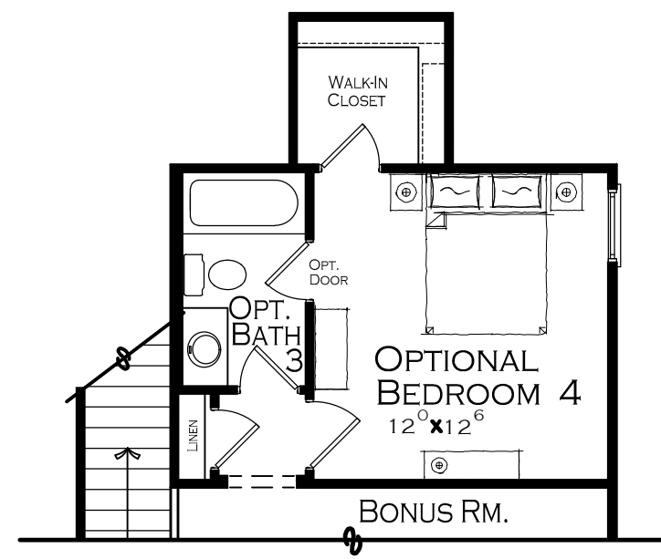
OPTIONAL BEDROOM #4 W/ OPT. FULL BATH #3 ADDITIONAL 270 SQ. FT.
