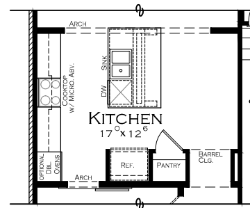
OPTIONAL KITCHEN 3 WITH OPT. DEEPER ISLAND WITH COOKTOP & MICRO. ABV. WITH BUILT-IN DBL. OVENS
