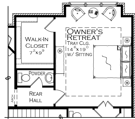
OPTIONAL ENLARGED OWNER'S RETREAT WITH SITTING AREA WITH 2' EXTENSION ADDITIONAL 64 Sq. Ft.
