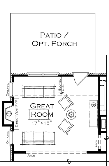
OPTIONAL F/P ON OUTSIDE WALL
