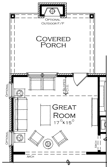
OPTIONAL REAR PORCH WITH OPT. EXTERIOR FIREPLACE
