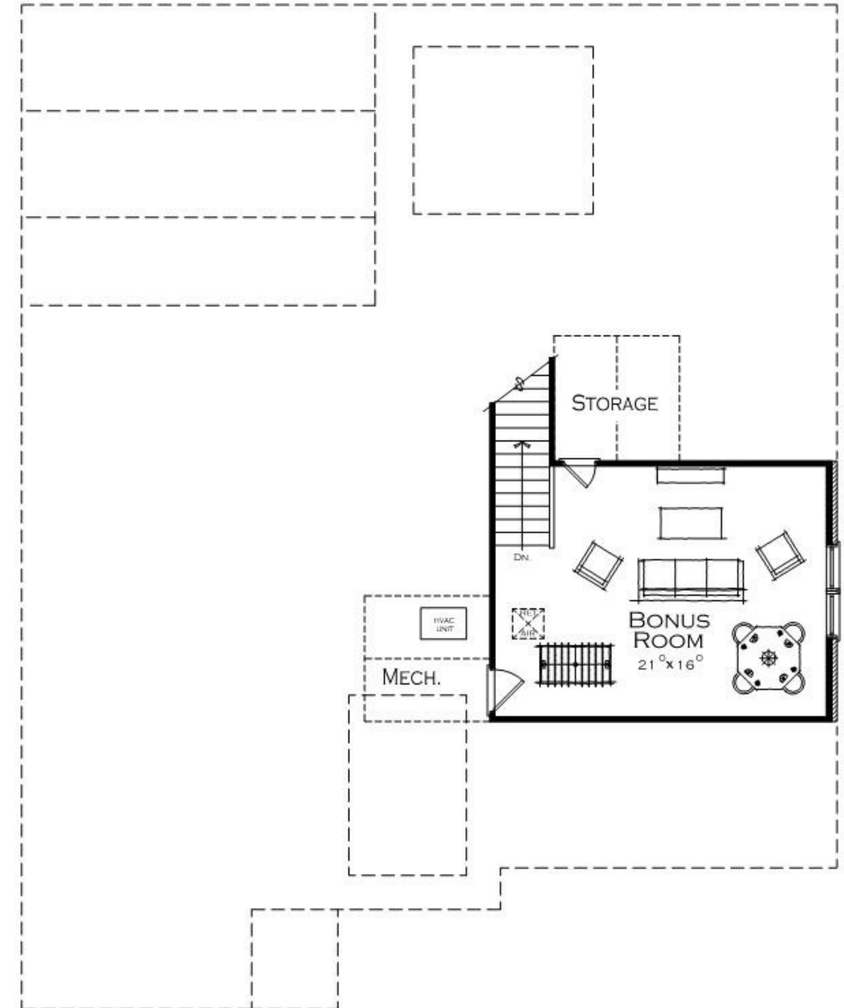
UPPER LEVEL
